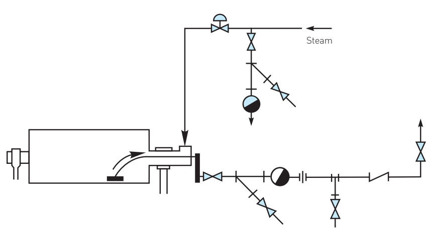
Rotating cylinder dryer (syphon drained)
