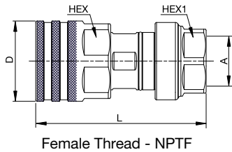
Female Thread - NPTF
