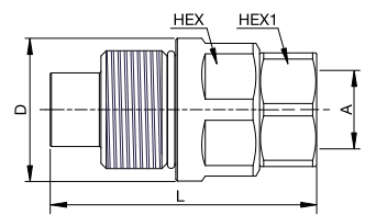
Female Thread - NPTF
