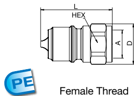
Female Thread
