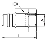
Female Thread
