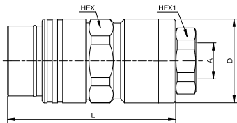
Female Thread - BSPP
