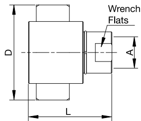
Female Thread
