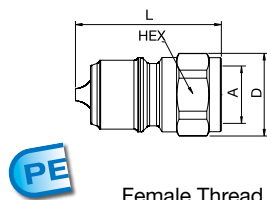
Female Thread
