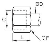
Nut 0110 and 0110..40
